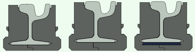
QTrack® SP Grooved rail QTrack® HP Grooved rail QTrack® XP Grooved rail
