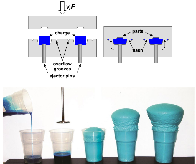
Figure 7: Stable compression moulding (top), compared to unstable foaming process (bottom)
