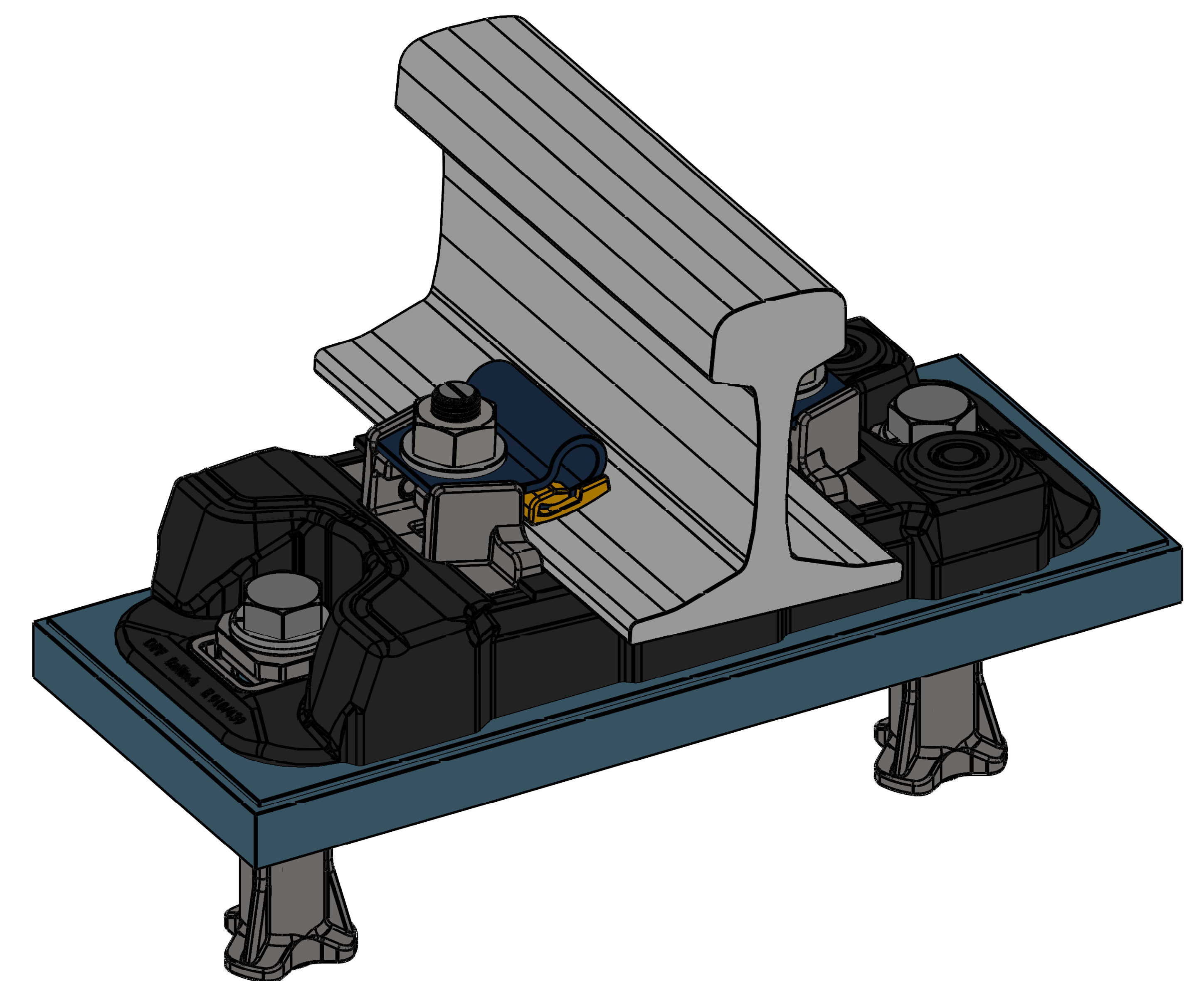
ISOMETRIC VIEW
